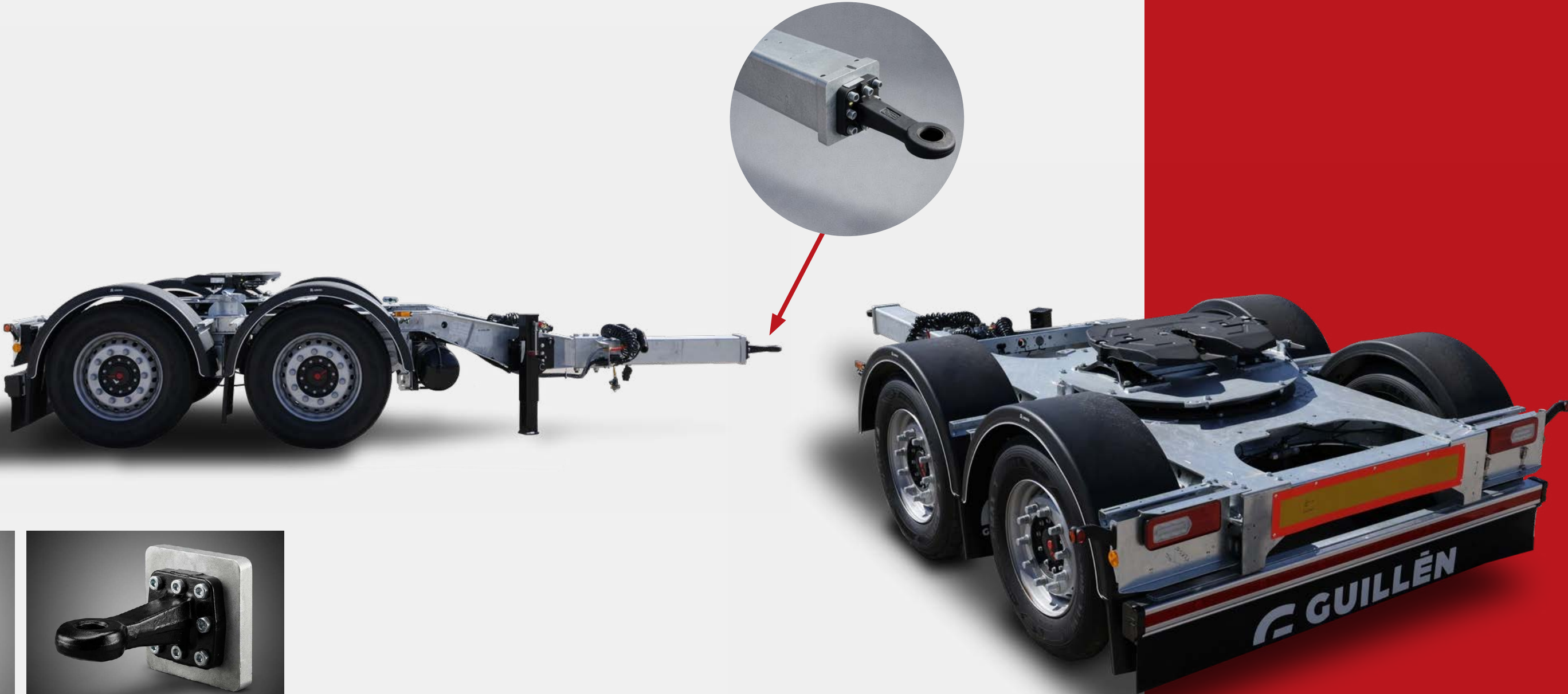
Drawbar end.
